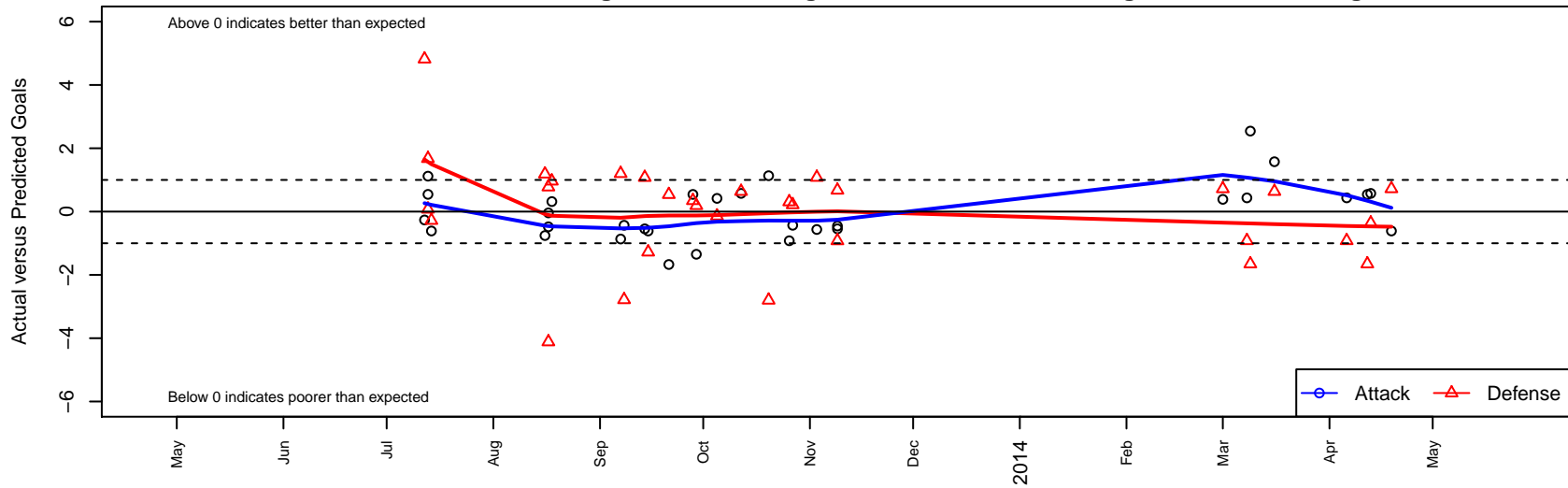
PCU SESC Furies G99 Dots are actual minus expected GF (blue circles) and GA (red triangles). Blue line is smoothed change in attack strength. Red is smoothed change in defense strength.
